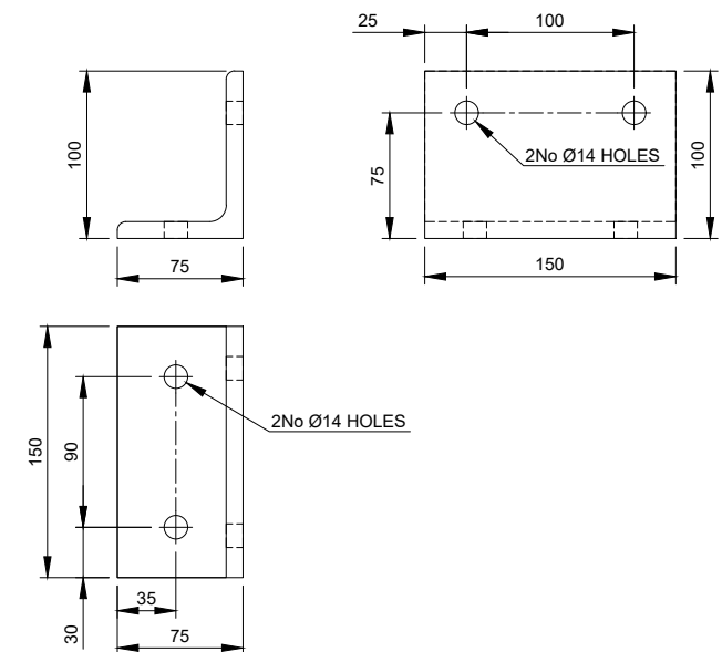
PART TPL-A-3 - UA100x75x10 Scale 1:5
