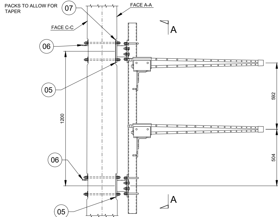
DETAIL G - Rx ANTENNA MOUNT SCALE 1:20
