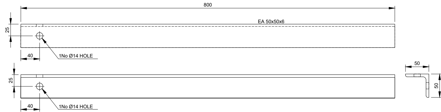
TPB-BR-1 - EA50x50x6 Scale 1:5
