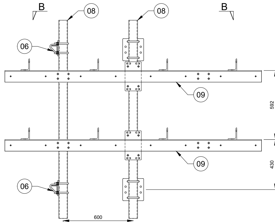
VIEW A-A SCALE 1:20
