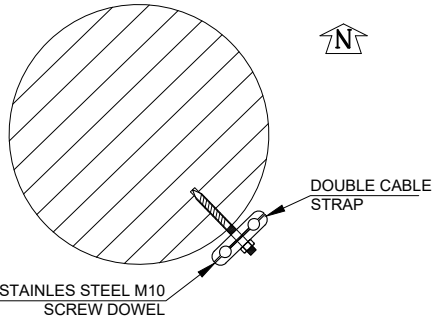
FEEDER MANAGEMENT Scale 1:10
